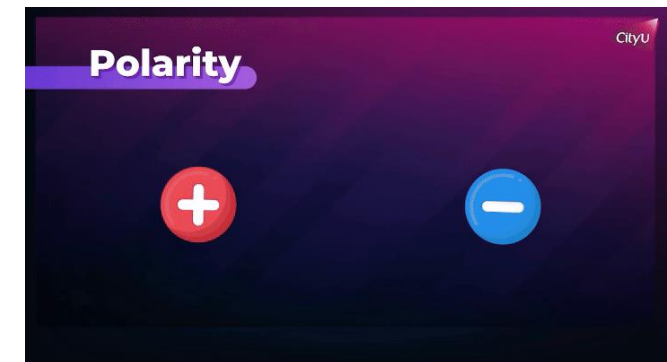
Animated Videos
